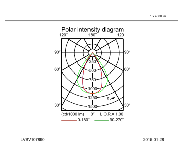
4MX400 G3 581 1xLED40S/840 PSD NB
