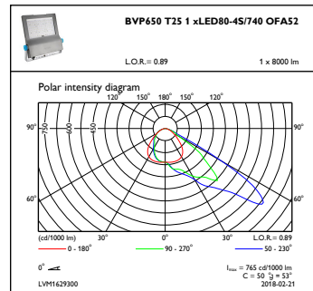
OFPC1_BVP650T251xLED80-4S740OFA52
