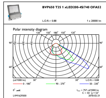
OFPC1_BVP650T251xLED200-4S740OFA52
