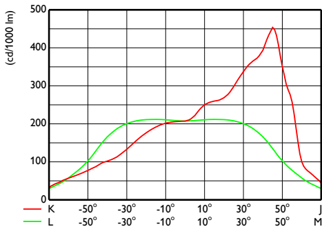
OFCS1_BVP650T251xLED200-4S740OFA52
