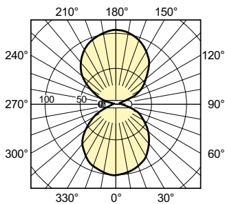
Light Distribution Diagram - MST SON-T PIA Plus 250W E40 1SL/12
