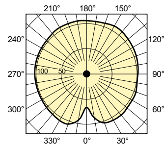
Light Distribution Diagram - MST SON-T PIA Plus 250W E40 1SL/12
