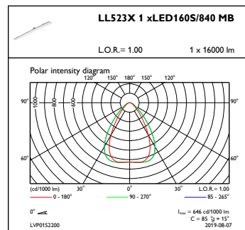
OFPC1_LL523X1xLED160S840MB
