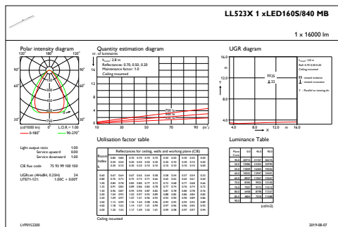
IFGU1_LL523X1xLED160S840MB
